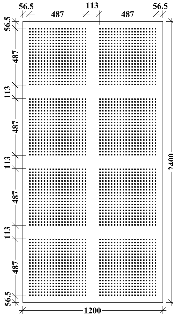
BIG Curve Quattro 41 with the measurement of 1200 x 2400 mm
