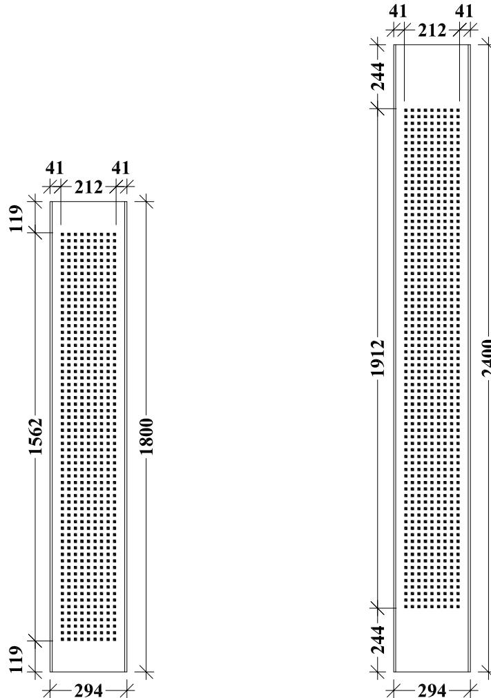
Plank with the actual size of 294 x 1800 mm and 294 x 2400 mm
