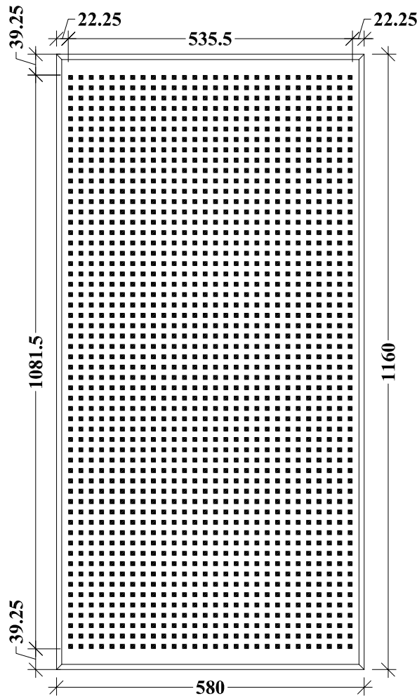
Trap modular size 580 x 1160 mm
